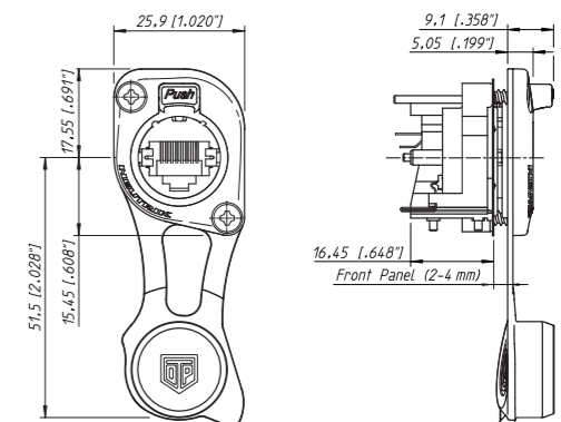
NE8FDV-TOP
