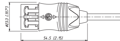
NKHDMI-*
