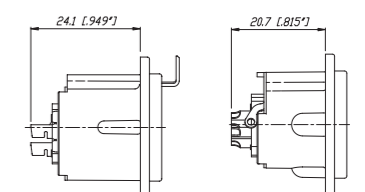
NC*MD-LX
