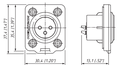
NC*MDX-TOP
