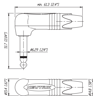
NP2RX
